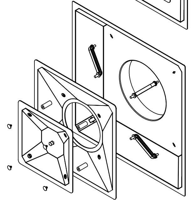
EXPLODED VIEW
